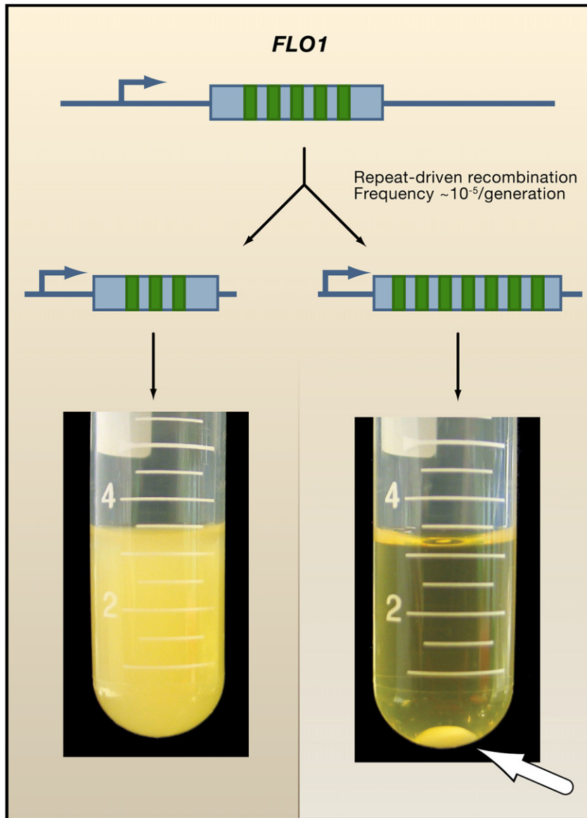
Figure 2. Recombination in Intragenic Repeats
